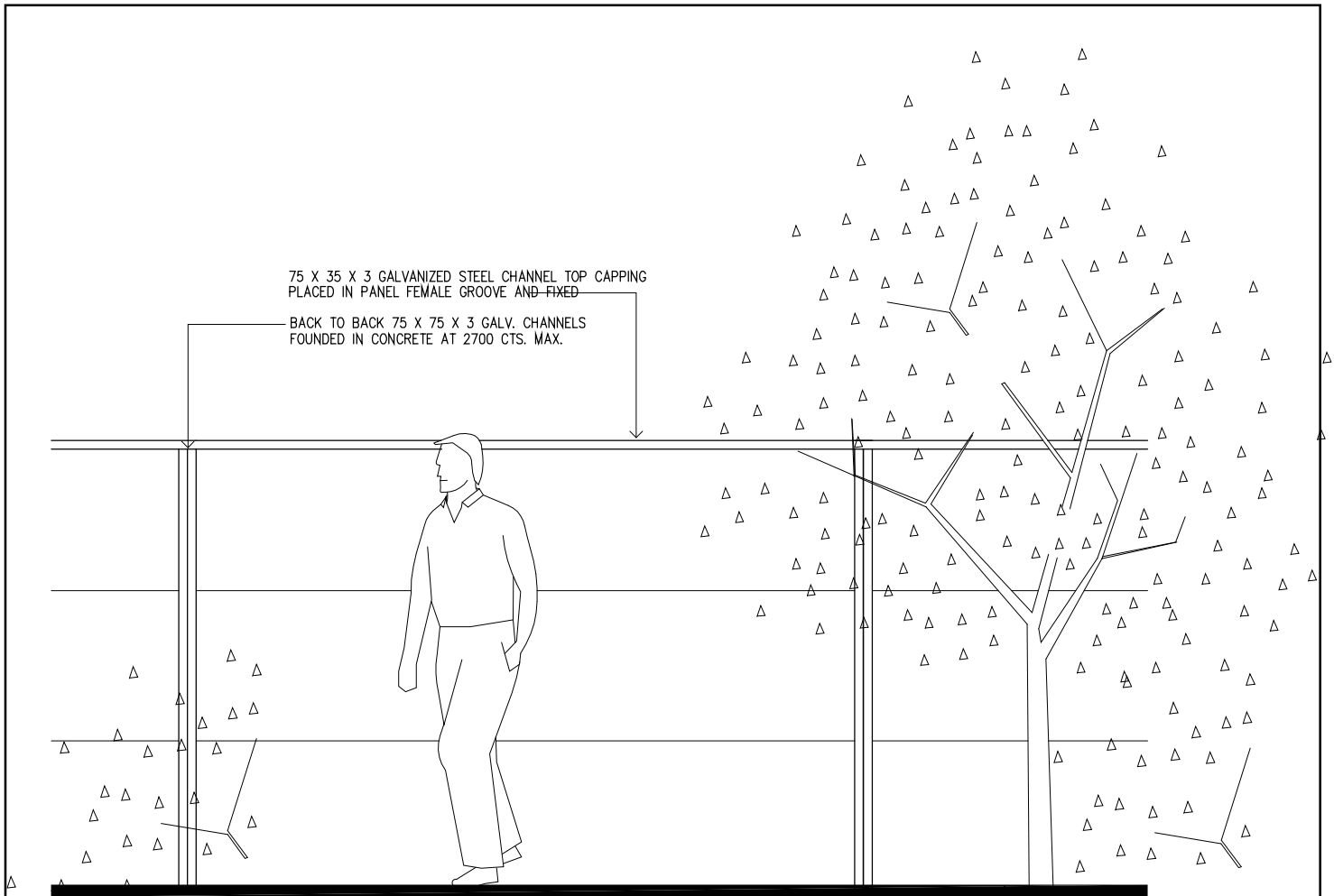
ELEVATION OF EXTERNAL FENCE FORMED WITH PANELS HORIZONTALLY PLACED
